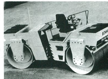
Bomag BW 161 AD tandem vibratory asphalt roller
